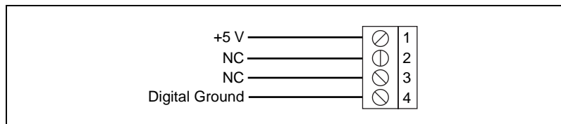
Figure 32. 4-Position Power Input Terminal Block Pin Assignment
