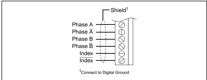
Figure 4. Differential Encoder Wiring
