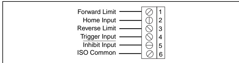
Figure 39. UMI-Flex4 Limit Switch Terminal Block Pin Assignment
