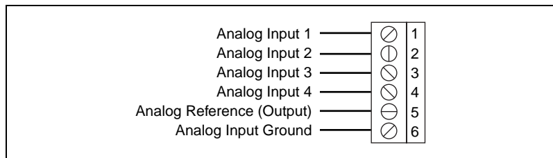
Figure 40. UMI-Flex4 Analog Input Channels 1 through 4
