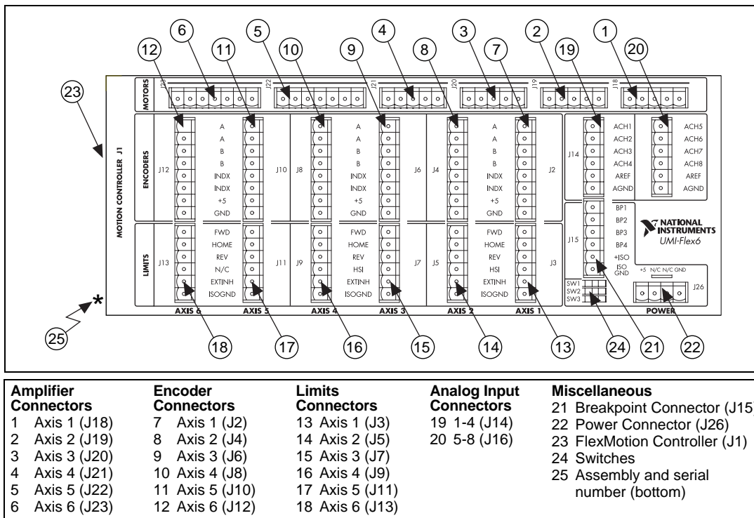
Figure 23. UMI-Flex6 Parts Locator Diagram
