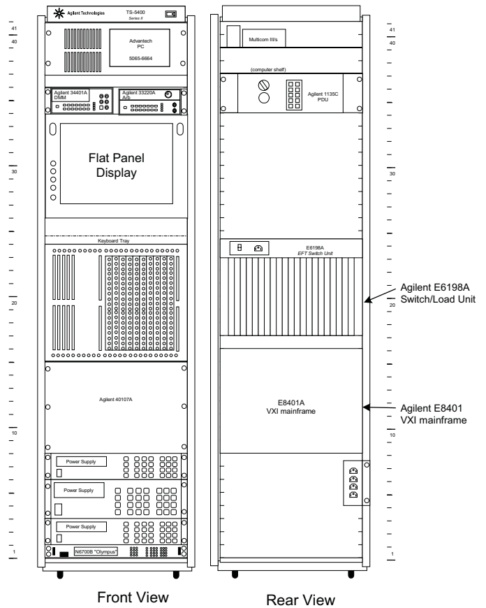
Figure 4: VXI/GPIB Mac Panel (front view and rear views)
